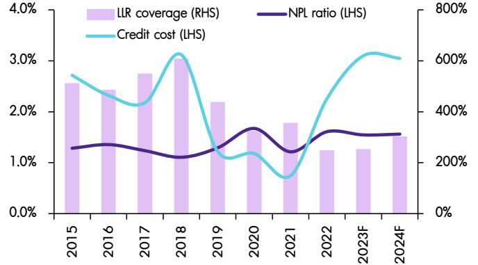
Figure 6: Asset quality
